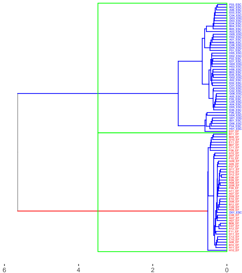
Hierarchical clustering
