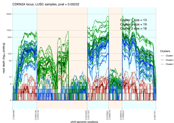
Figure 2: Graphical output from Sffigure for lpplots=2 . The curves are colored according to class label. The red curves represent a low expression class. There is a large difference in expression of the second exon between the blue and green curves. This difference is reflected in the highly significant p -value.
