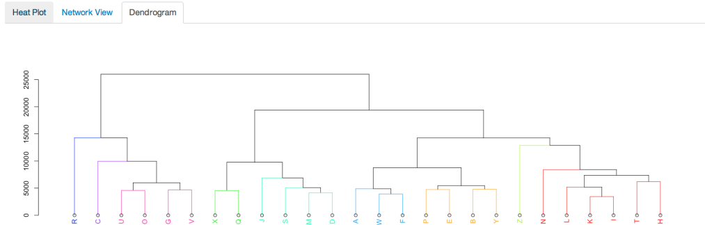
Figure 26: Dendrogram - Samples
