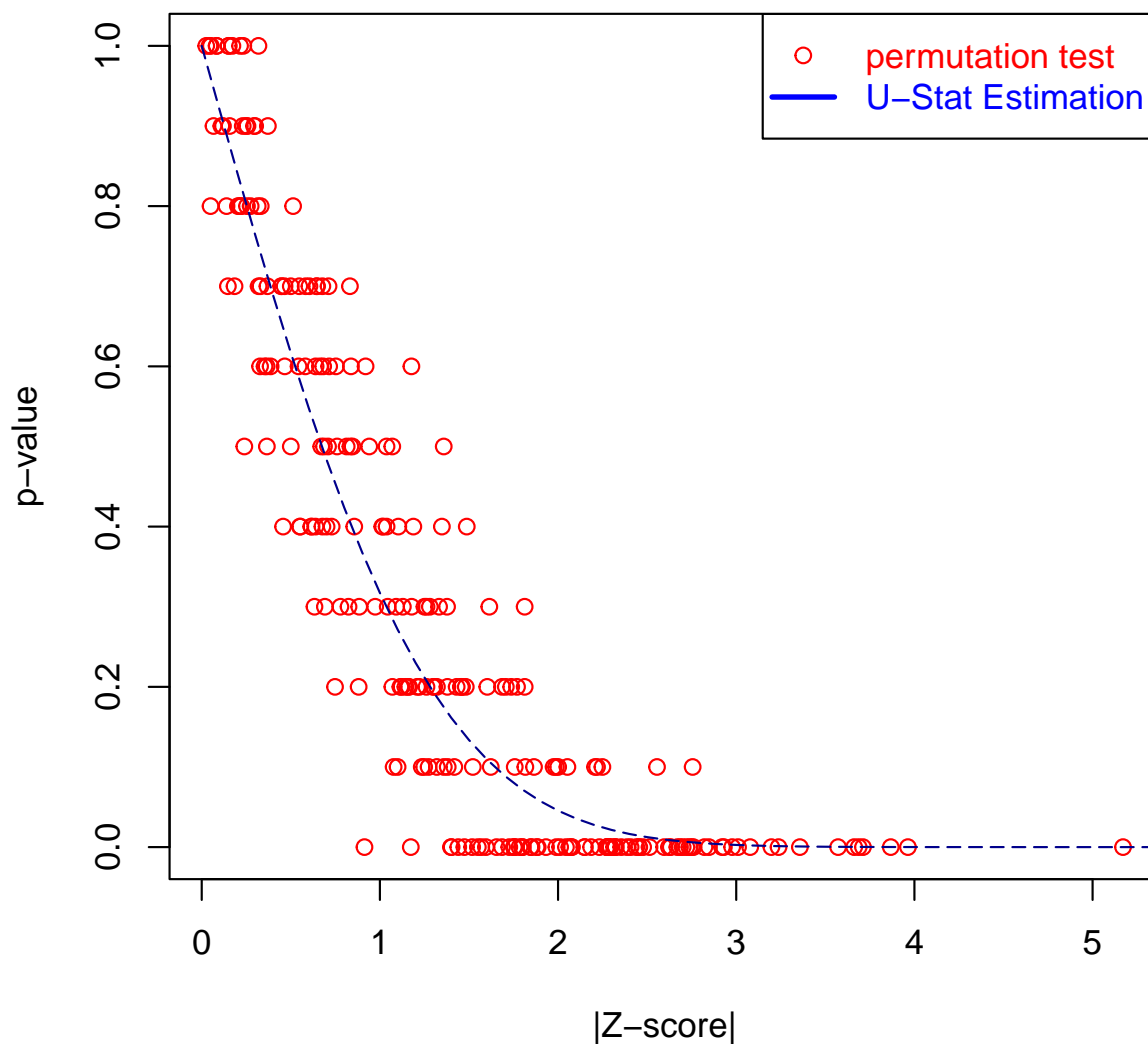
Figure 3: Comparing p-value from permutation test and U-statistic theory with only 10 permutations.
