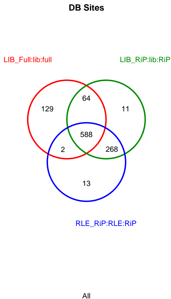
Figure 19: Venn diagram showing overlapping differentially bound sites identified in analyses using library-size normalization with full and reads-in-peaks library sizes, as well as RLE normalization using reads-in-peaks
