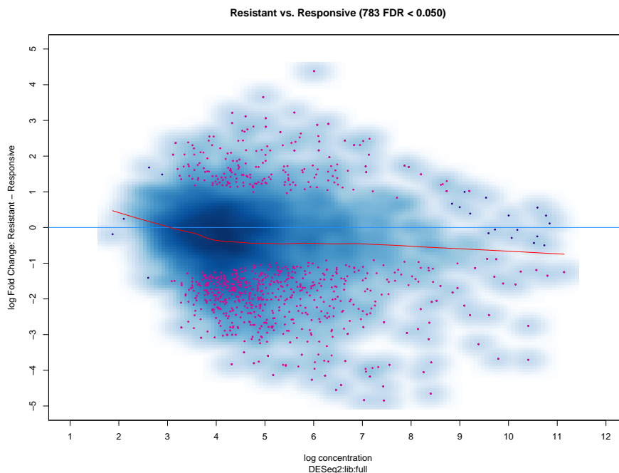
Figure 15: MA plot showing results of analysis using Library-size based normalization
