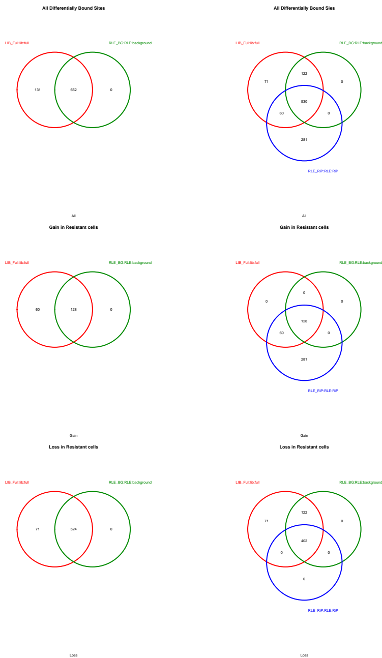
Figure 21: Venn diagrams of overlapping differentially bound sites identified using full library size based normalization compared to background RLE and Reads in Peaks RLE normalization
