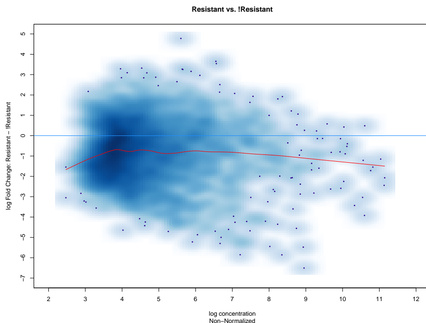
Figure 14: MA plot showing non-normalized data Generated by plotting the result of: dba.plotMA(tamoxifen, contrast=list(Resistant=tamoxifen$masks$Resistant), bNormalized=FALSE, sub="Non-Normalized")
