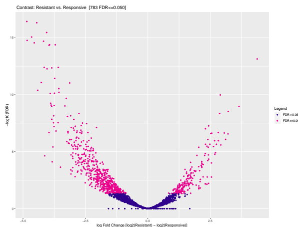
Figure 12: Volcano plot of Resistant-Responsive contrast, using a multi-factor design "Tissue + Condition"
