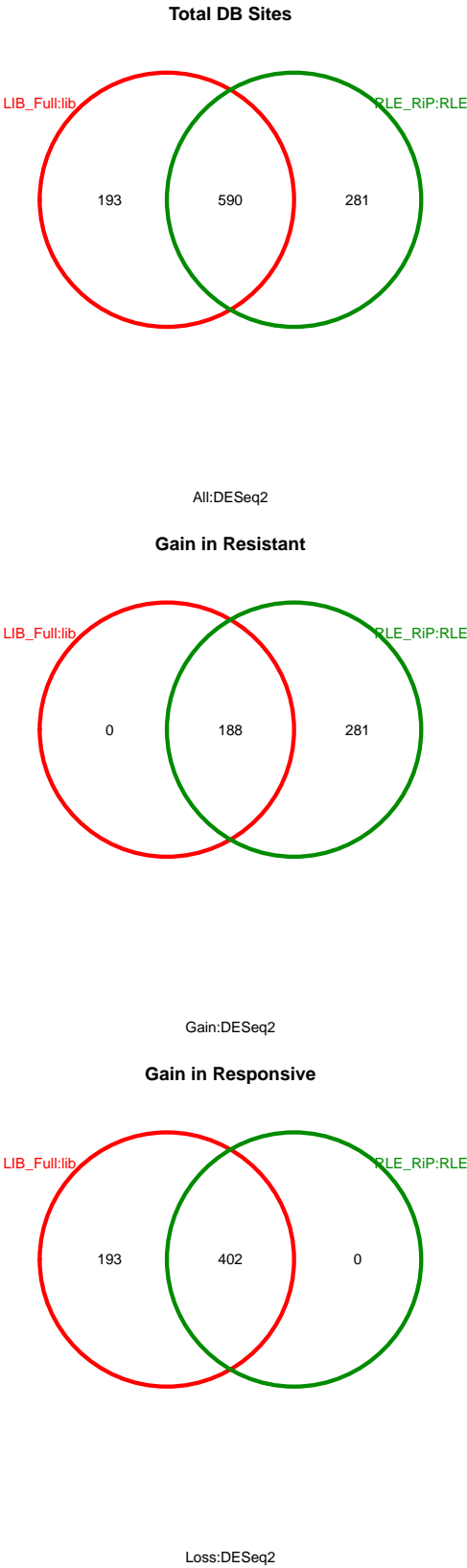
Figure 17: Venn diagrams showing overlaps of sites identified as differentially bound when using library size vs RLE normalization
