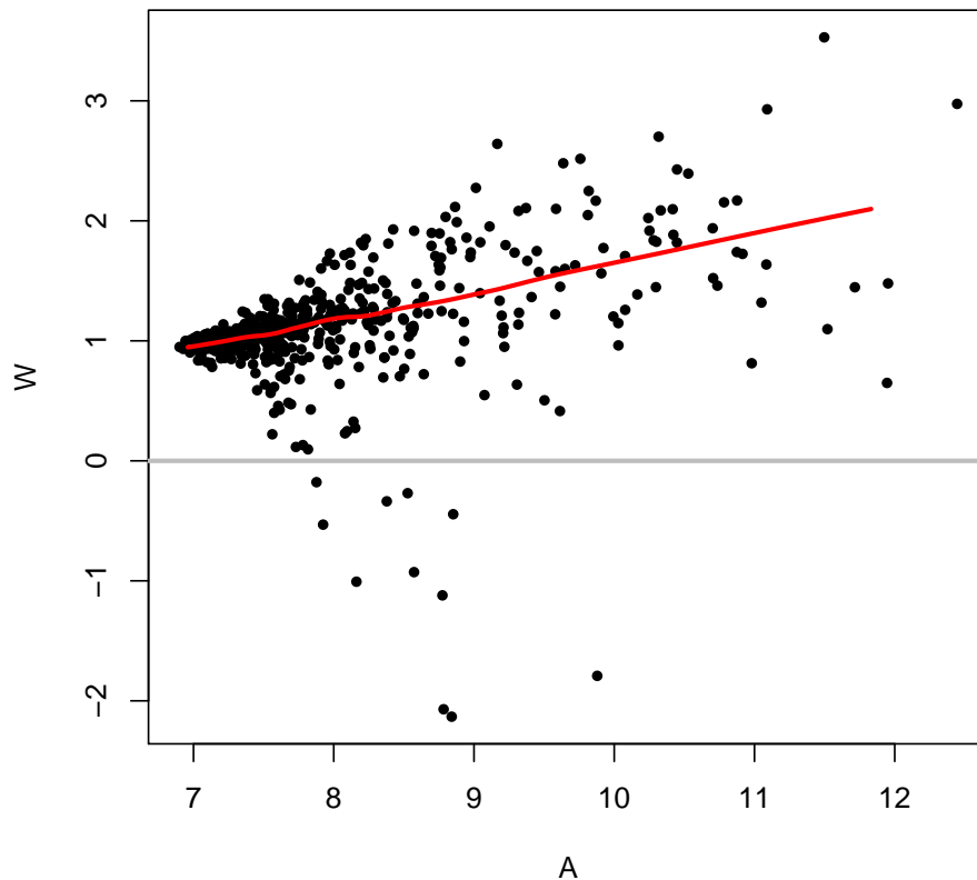
Figure 1: WA plot for the first chip of the gastro data.
