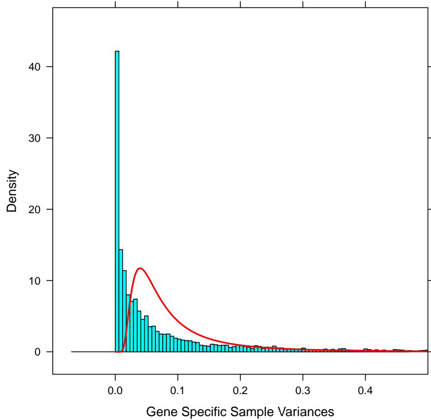
Figure 8: Density histogram of gene specific sample variances and the scaled inverse chi-square density plot (red line).
