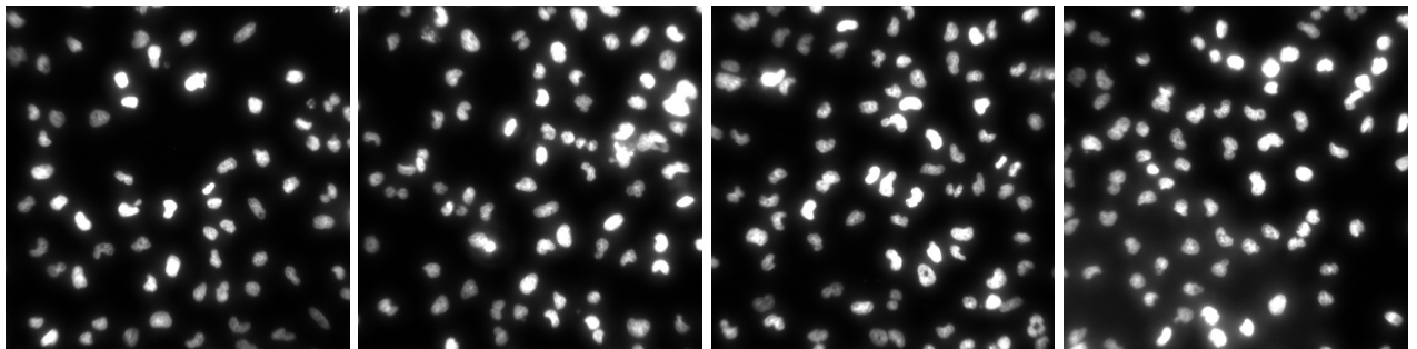
Figure 17: nuc
