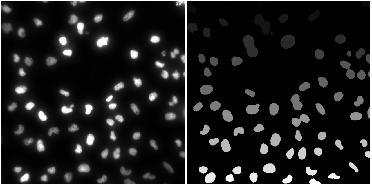
Figure 13: nuc[ , ,1] , nuclabel/max(nuclabel)
