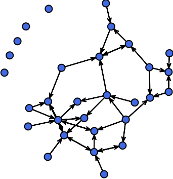
Priors weight = 0.25
