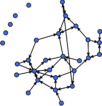
Priors weight = 0.75
