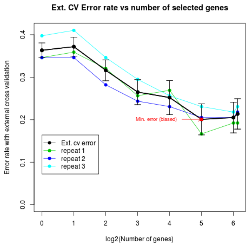
Figure 4.2: Cross-validated error rate averaged over the repeats .
