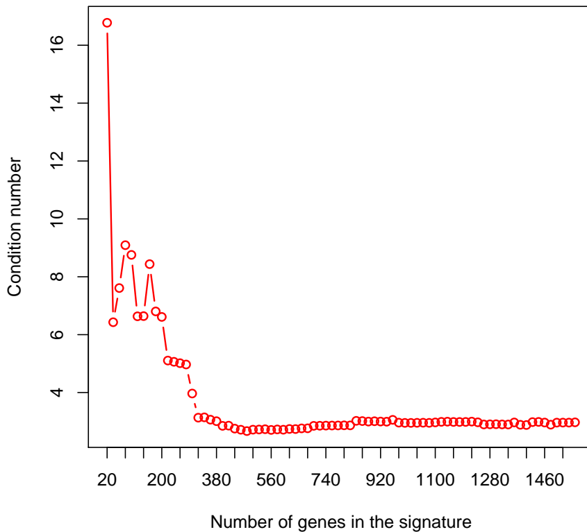
Condition number of the signature matrix
