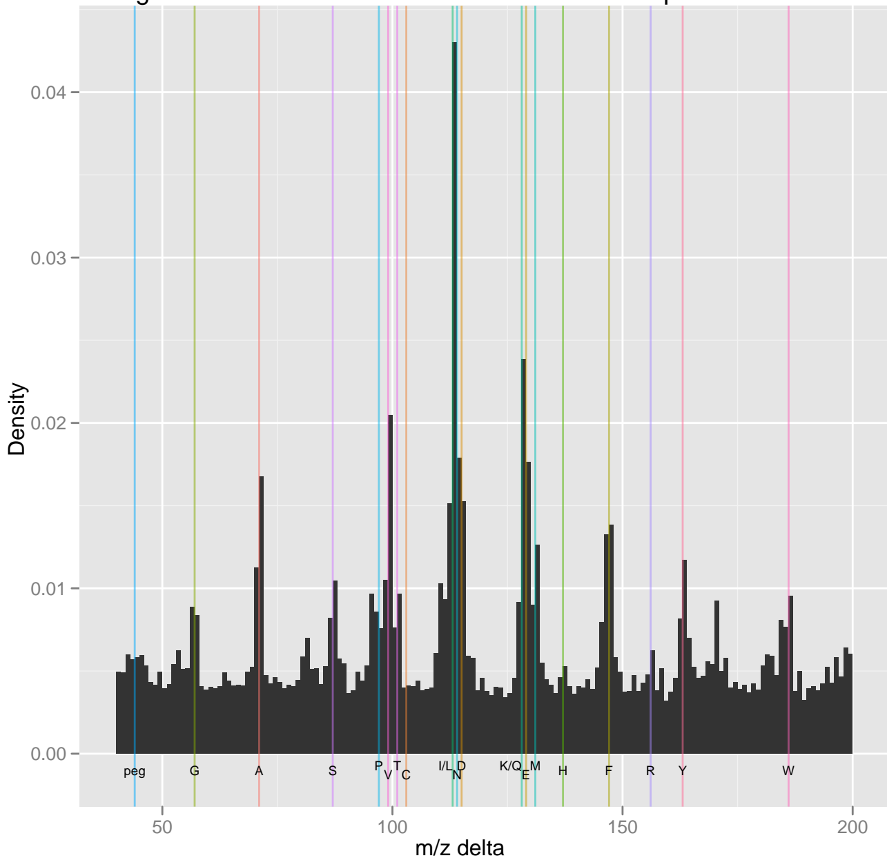
Histogram of Mass Delta Distributions for PRIDE experiment 12011
