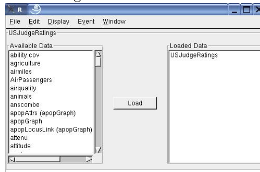
Figure 2: Loaded Data
