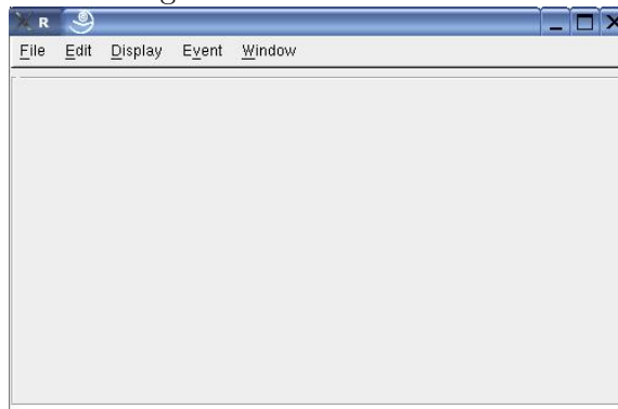
Figure 1: Control Window
