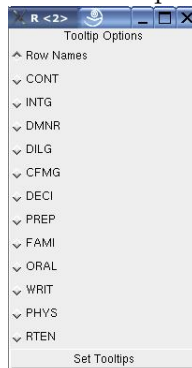
Figure 15: Tooltip Options
