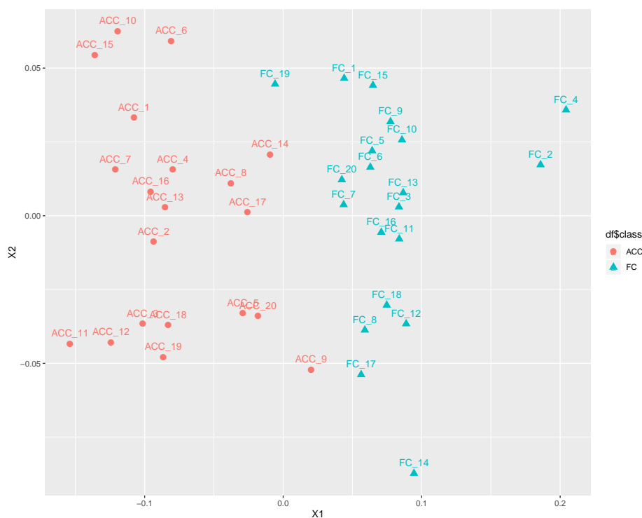
Figure 9: MultiDimensional Scaling plot A MDS plot is drawn, considering only most informative genes, obtained after feature selection: color code is referred to 'class'.
